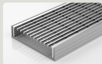
100TRG20 Standard Grate 3mm wire/5mm gap 106mm x 23mm DN40 / DN50 / DN80 / DN100
