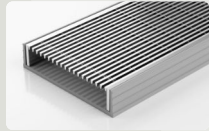
100ARG20 Premium Grate 2mm wire/2.5mm gap 106mm x 23mm DN40 / DN50 / DN80 / DN100
