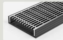
100TRGBL20 Standard Grate 3mm wire/5mm gap 106mm x 23mm DN40 / DN50 / DN80 / DN100
