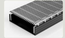
100ARGBL30 Premium Grate - Channel Overlay 2mm wire/2.5mm gap 106mm x 32mm DN40 / DN50 / DN80 / DN100
