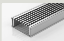
65TRG25 Standard Grate 3mm wire/5mm gap 74mm x 27mm DN40 / DN50
