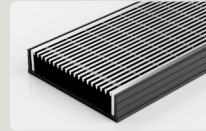
100ARGBL20 Premium Grate 2mm wire/2.5mm gap 106mm x 23mm DN40 / DN50 / DN80 / DN100
