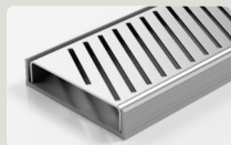
100PASG20 Punched Angle Design 106mm x 23mm DN40 / DN50 / DN80 / DN100
