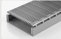
100ARG30 Premium Grate - Channel Overlay 2mm wire/2.5mm gap 106mm x 32mm DN40 / DN50 / DN80 / DN100
