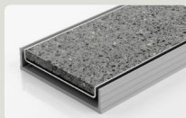
100TiG20 Tile Insert Tiles up to 10mm Deep 106mm x 23mm DN40 / DN50 / DN80 / DN100
