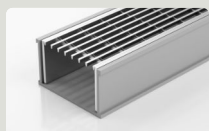
65TRG40 Standard Grate 3mm wire/5mm gap 74mm x 42mm DN40 / DN50
